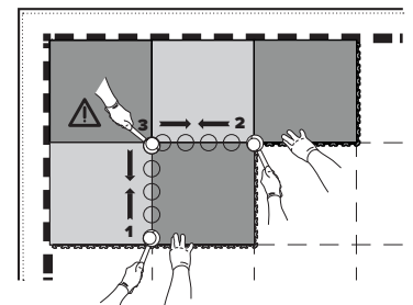
Fig. 4 Method of installing INVISIBLE, INVISIBLE XL, BUSINESS
